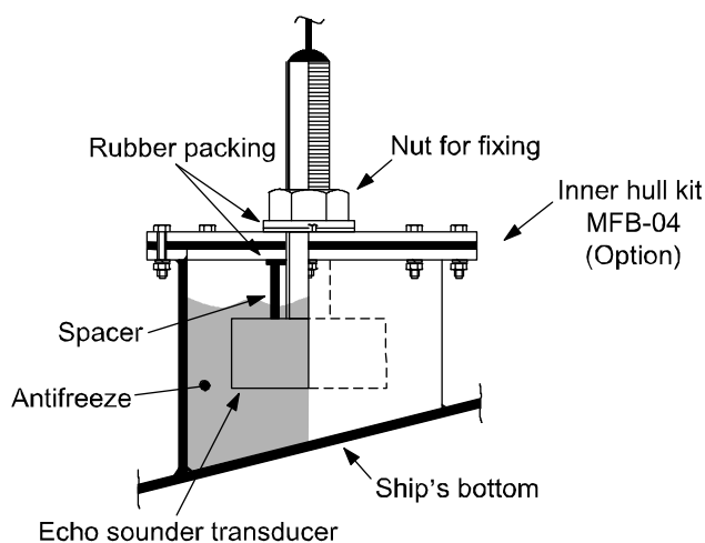
Figure 5.6 Inner-hull installation
