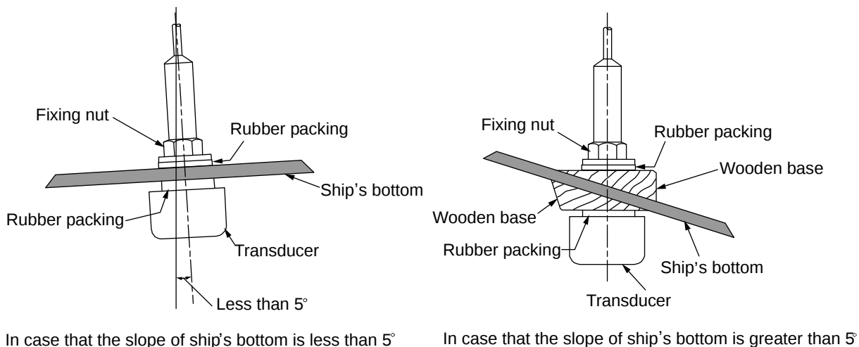
Figure 5.7 Through-hull Installation
