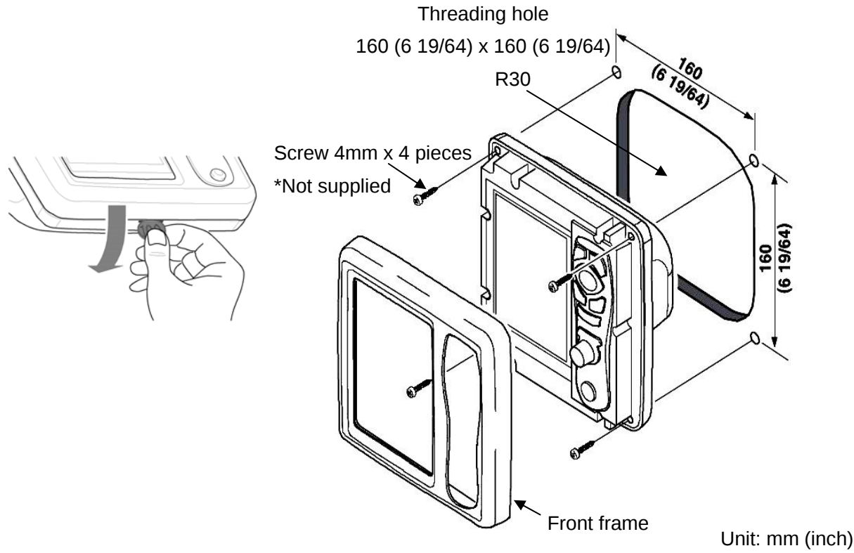
Figure 5.3 Flush-mount Installation
